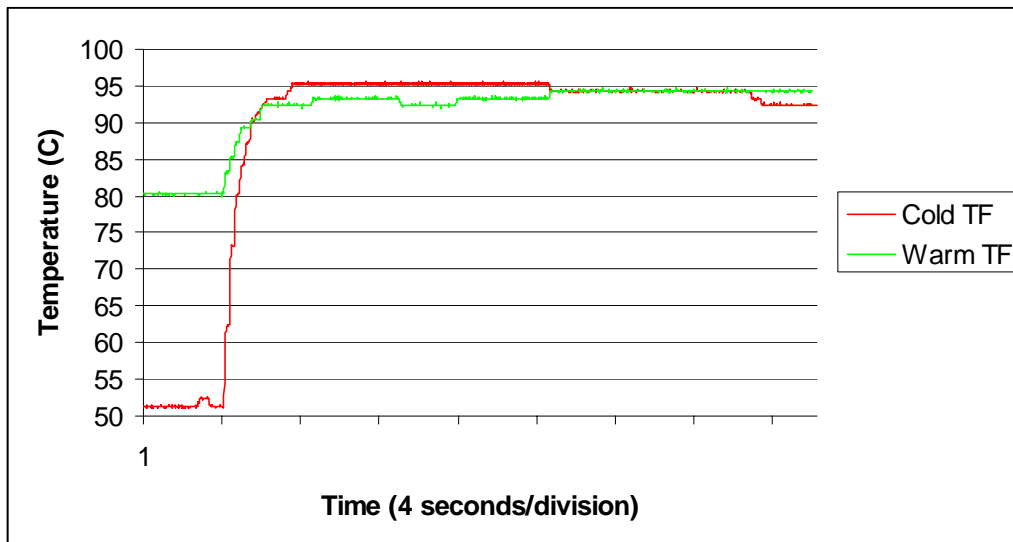
Figure 10. Waveform difference between a cold & dry Thermofilter and a warm & wet Themofilter. The cold Thermofilter was soaked in tap water before mounted to the grouphead. It was equilibrated to 31°C before mounting to the grouphead. However, the heat at the grouphead quickly warms the sensor tip in the Thermofilter to 51°C before the shot was pulled (as shown in the figure). As we can see that the average temperature will be very different than the peak temperature.
